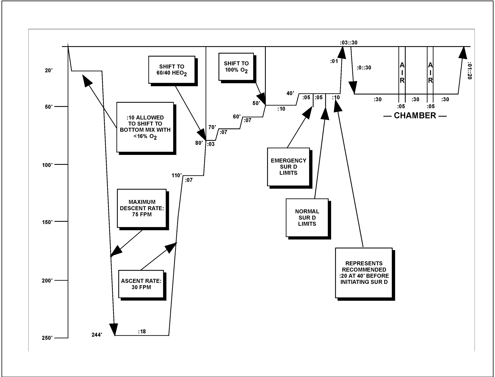
Figure 14-4. Normal Surface Decompression Dive Profile for a 249 fsw/:18 Dive.
